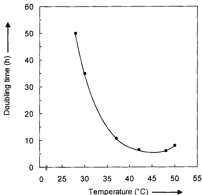
Fig. 41. Effect of temperature on doubling time of Trimyema minutum strain EV10. No growth was observed below 28 °C and above 52 °C.
