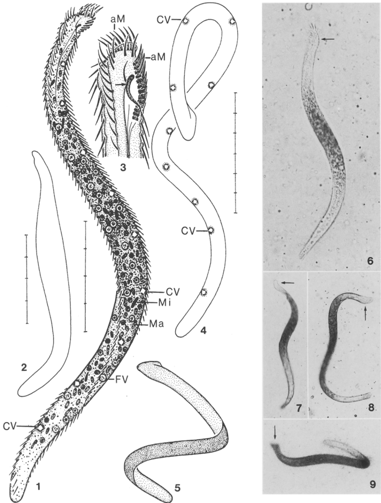
Figs. 1–9. Circinella arenicola from life. – Fig. 1. Ventral view of typical specimen. – Fig. 2. Lateral view of well-nourished trophont. – Fig. 3. Oral area of specimen with helmet-like anterior end. Arrow marks compact oral lip. – Figs. 4, 5. Slender theront and spiralized, slowly moving specimen. – Figs. 6–9. Bright field light micrographs of freely moving, typical specimens. Arrows mark broadened (cephalized) anterior end. The middle third of the cells contains many food vacuoles and thus appears dark. aM = adoral membranelles, CV = contractile vacuoles, FV = food vacuole, Ma = macronuclear nodule, Mi = micronucleus. Scale bar division = 20 µm.
