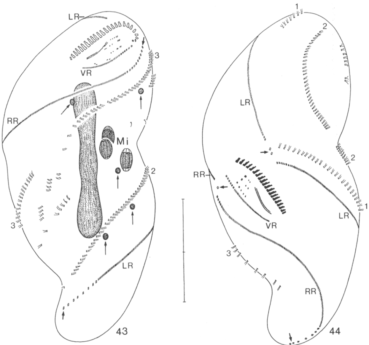
Figs. 43, 44. Circinella arenicola , middle morphogenetic stage, protargol impregnation. The opisthe's oral apparatus is almost complete and the anlagen in the proter and opisthe organize cirri. The dorsal kineties reproduce by intrakinetal proliferation of kinetids. Thick arrows mark parental marginal cirri. The macronuclear nodules have fused to a roundish mass which elongates to a dumb-bell-shaped structure; some degenerating macronuclear nodules are recognizable (thin arrows). The micronuclei commence division. LR = left marginal row, Mi = micronuclei, RR = right marginal row, VR = ventral cirral row, 1, 2, 3 = dorsal kineties. Scale bar division = 20 \mu m.
