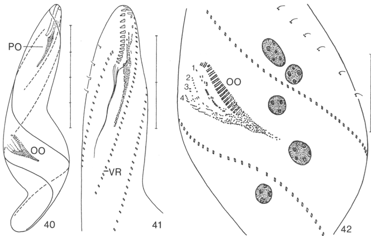
Figs. 40–42. Circinella arenicola , middle morphogenetic stage, protargol impregnation. The oral primordium of the proter (PO) unites with the anlagen organized by the frontal cirri and the undulating membranes. The oral primordium of the opisthe (OO) organizes adoral membranelles and four streaks of basal bodies (1–4). The parental ventral cirral row (VR) does not organize anlagen and thus appears unchanged. Scale bar division = 20 \mu\text{m} .
