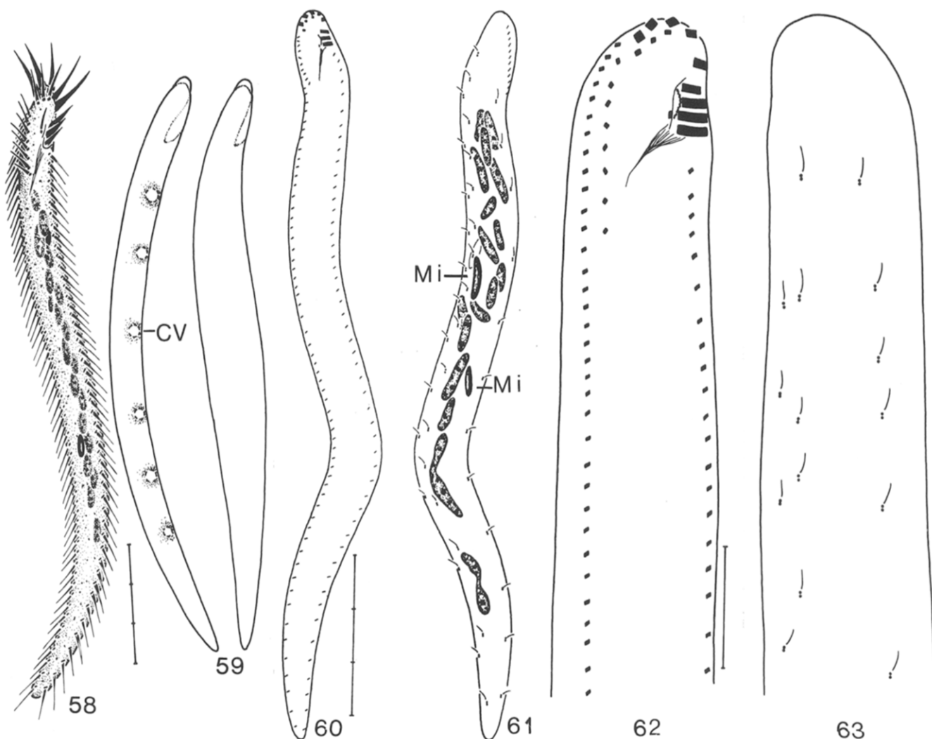
Figs. 58–63. Circinella vettersi from life (Figs. 58, 59) and after protargol impregnation (Figs. 60–63). – Fig. 58. Ventral view of a theront. – Fig. 59. Ventral view of a trophont. – Figs. 60, 61. Infraciliature of the ventral and dorsal side of a theront. – Figs. 62, 63. Infraciliature of the anterior ventral and dorsal side at higher magnification. CV = contractile vacuole, Mi = micronuclei. Scale bar division = 10 \mu m. Reproduced from [2].
