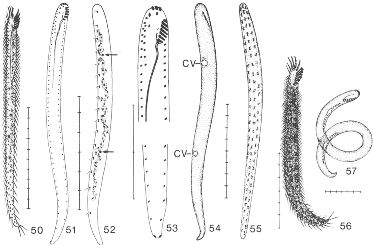
Figs. 50–57. Circinella filiformis from life (Figs. 50, 54–57) and after protargol impregnation (Figs. 51–53). – Figs. 50, 54. Ventral and dorsal view of theronts. – Figs. 51, 52. Infraciliature of the ventral and dorsal side of a theront. Arrows mark micronuclei. – Fig. 53. Ventral infraciliature at higher magnification. – Fig. 55. Lateral view of a theront. The cortex contains small crystals. – Figs. 56, 57. Ventral views of an extended and a spiralized trophont. CV = contractile vacuoles. Scale bar division = 10 \mu m. Reproduced from [9].
