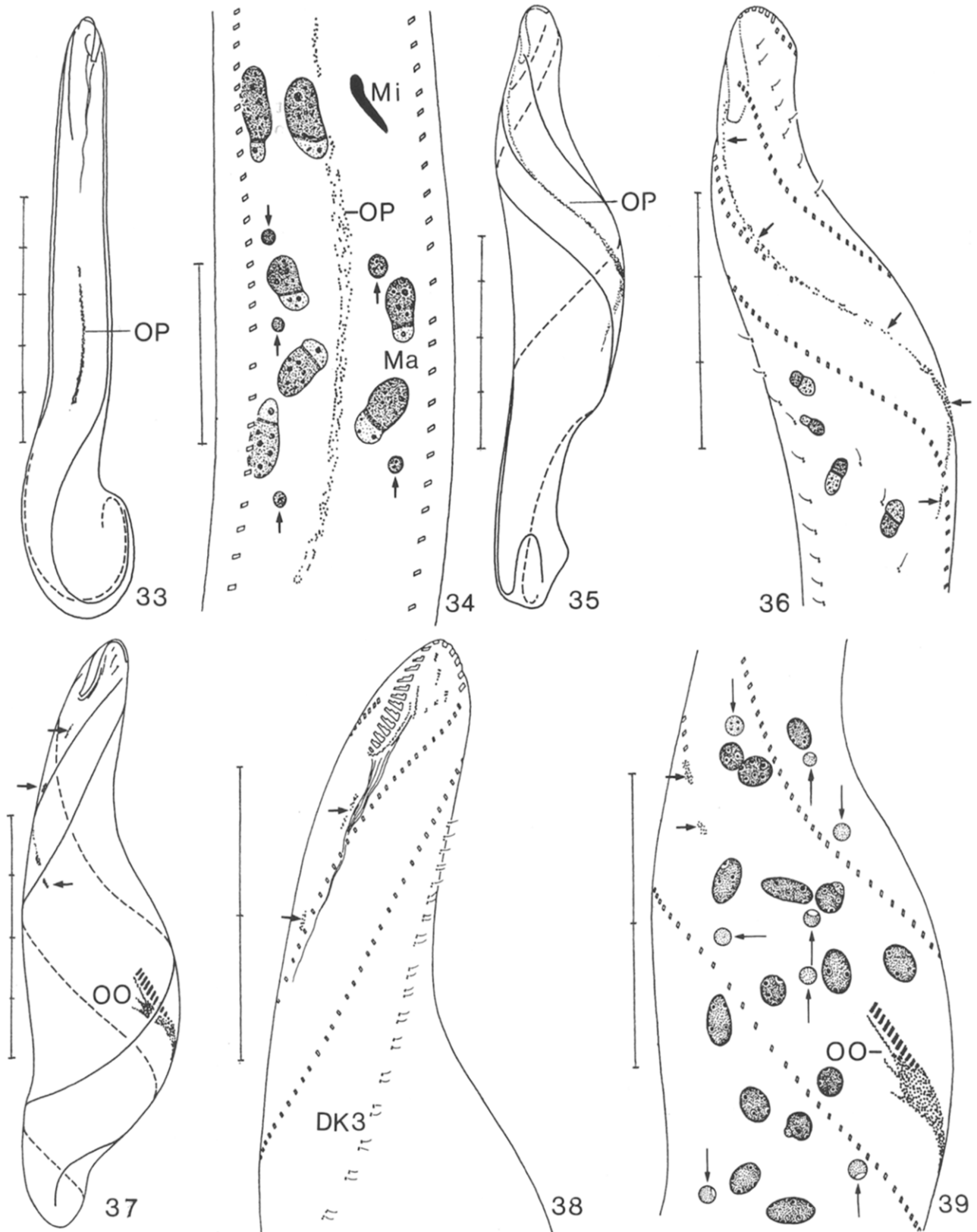
Figs. 33–39. Circinella arenicola , early morphogenetic stages, protargol impregnation. – Figs. 33, 34. Division commences with the apokinetal development of an oral primordium in mid-body. The posterior portion of the cell shortens and rounds up. Some macronuclear nodules degenerate (arrows). – Figs. 35, 36. The oral primordium develops to a long streak of basal bodies extending from mid-body to proter's oral apparatus (arrows). The middle portion of the cell broadens. – Figs. 37–39. The oral primordium divides into an anterior (thick arrows) and posterior portion (OO). The proter's frontal cirri and undulating membranes organize cirral anlagen. Many macronuclear nodules degenerate (thin arrows). DK3 = dorsal kiny 3, Ma = macronuclear nodule, Mi = micronucleus, OO = opisthe's oral apparatus, OP = oral primordium. Scale bar division = 20 μm.
