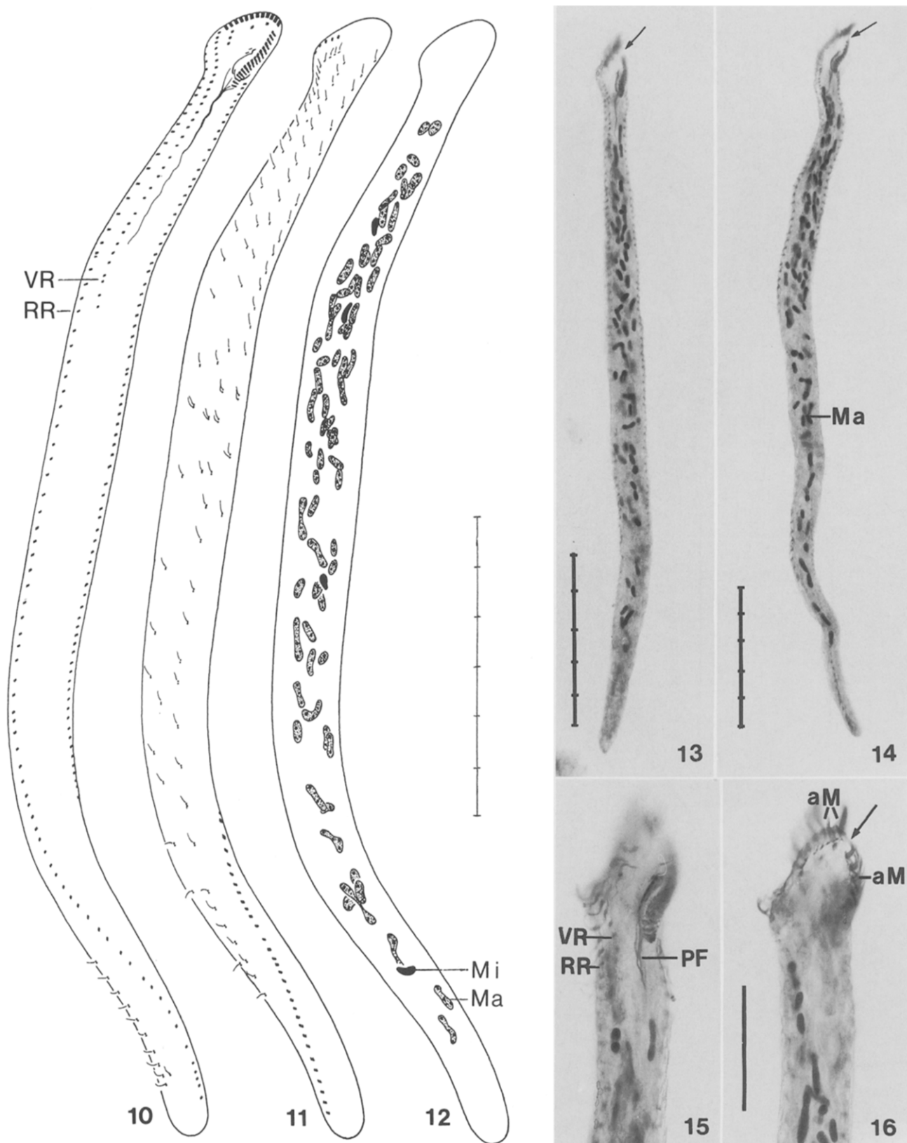
Figs. 10–16. Circinella arenicola after protargol impregnation. – Figs. 10–12. Infraciliature of ventral and dorsal side, and nuclear apparatus. – Figs. 13, 14. General morphology. Arrows mark break between distal and proximal adoral membranelles. – Figs. 15, 16. Anterior portion of single specimen photographed at two focus levels to show broadened (cephalized) oral area, ventral cirral row, and break between distal and proximal adoral membranelles (arrow). aM = adoral membranelles, Ma = macronuclear nodule, Mi = micronucleus, PF = pharyngeal fibers, RR = right marginal row, VR = ventral cirral row. Scale bar division = 20 µm. Note: To save space, all figures are orientated as seen from the ventral side, i.e. the dorsal surface is shown by transparency. In the spiralized dividers the opisthe's oral apparatus always faces the observer.
