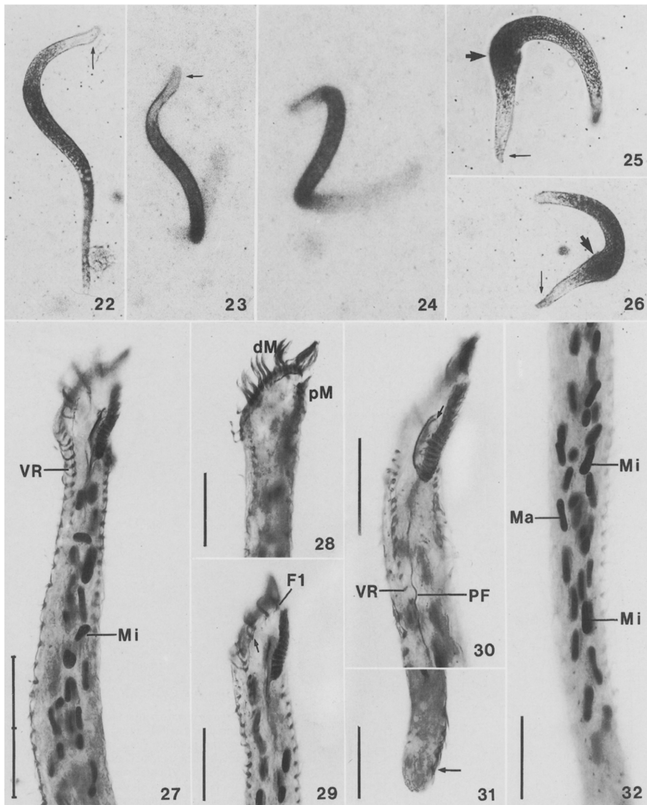
Figs. 22–32. Circinella arenicola in vivo (Figs. 22–26) and after protargol impregnation (Figs. 27–32). – Figs. 22–24. Bright field light micrographs of freely moving, typical specimens. Arrows indicate anterior end of cells. – Figs. 25, 26. Lateral view of specimens with bulbous broadening (thick arrows). Thin arrows mark flattened anterior end. – Figs. 27, 28. Ventral views of broadened (cephalized) anterior body portion. – Fig. 29. Anterior end of indistinctly cephalized specimen. Arrow marks single cirrus below 3rd frontal cirrus. – Fig. 30. Oblique ventral view showing spoon-shaped endoral membrane and shallow depression nearby (arrow; cp. Fig. 21). – Fig. 31. The marginal cirral rows end subterminally (arrow). – Fig. 32. Middle portion of cell showing two comma-shaped micronuclei and many macronuclear nodules. dM = distal adoral membranelles, F1 = first frontal cirrus, Ma = macronuclear nodule, Mi = micronuclei, PF = pharyngeal fibers, pM = proximal adoral membranelles, VR = ventral cirral row. Scale bar division = 20 \mu m.
